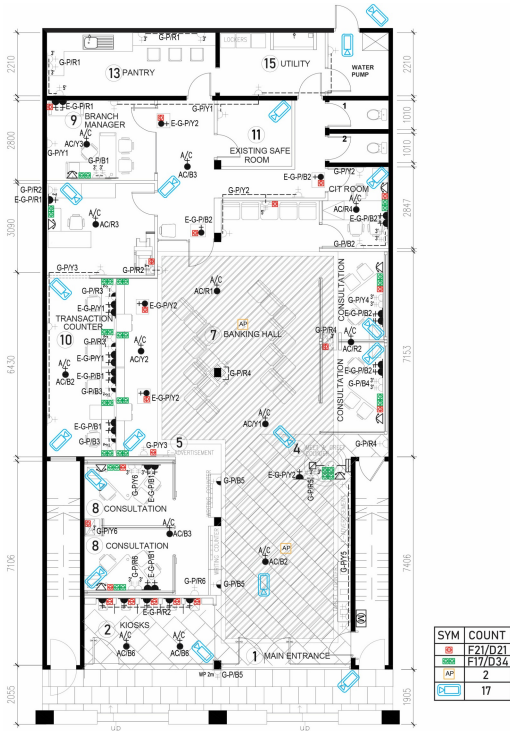
Ground Floor Plan - FACEPLATES & DATA POINTS Scale 1:150 (A3)
